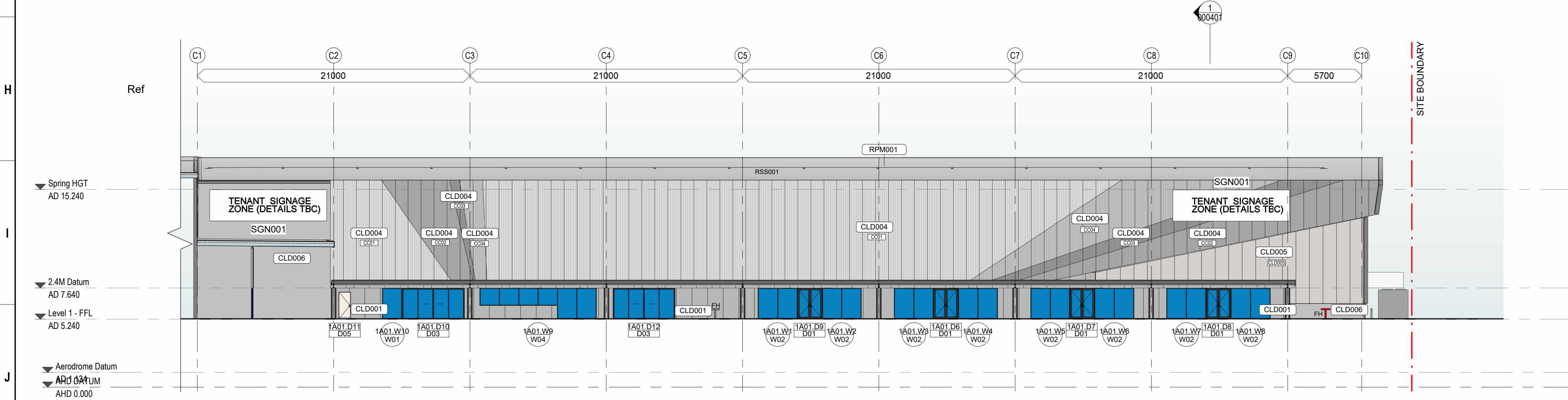
3 SOUTH EAST - PART C 1 : 200
