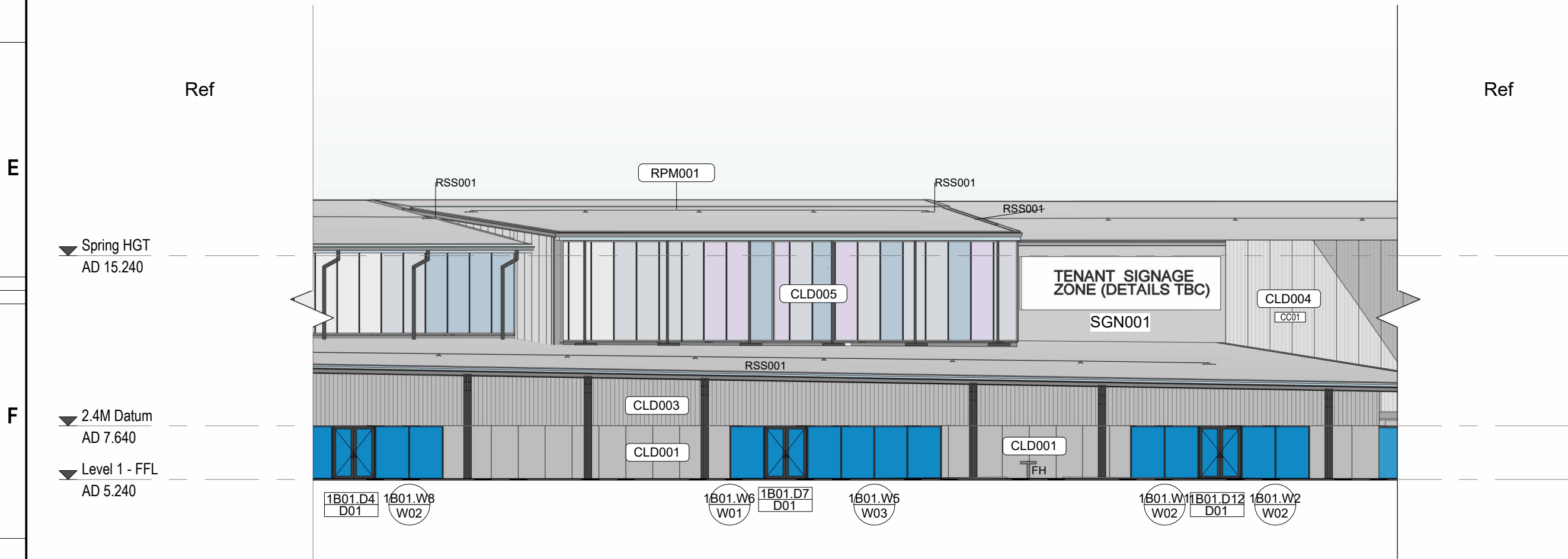
2 SOUTH EAST - PART B 1 : 200
